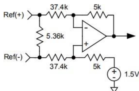
Figure 4.3.1 Analog hardware input circuit
