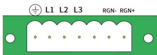
Figure 2.1 European Standard Terminal Sockets
