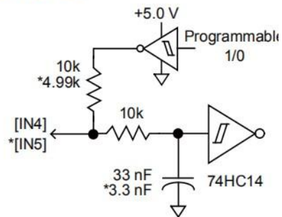
Figure 4.4.2 IN4-IN5 hardware input circuit
