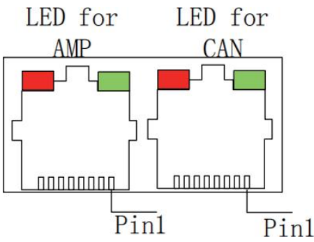
图2.6 RJ45 8针水晶头座
